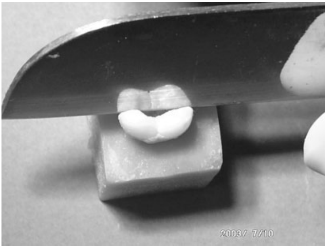
Figure 1. The lingual cusps of the teeth were standard fractured at the cemento-enamel junction using a sharp indenter.
